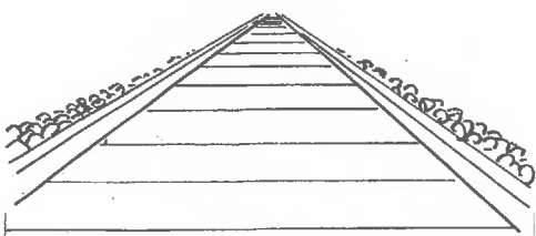
せんろ
